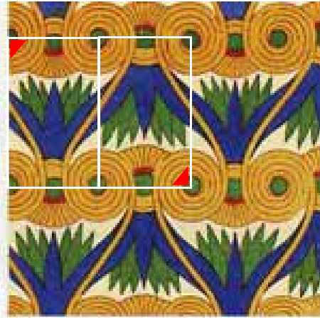
6 - sym 3 (pm)
